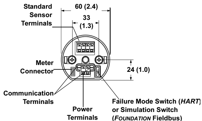
Shown with Standard Compression Screw Terminals
