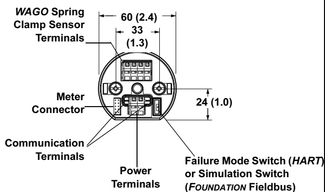
Shown with WAGO® Spring Clamp Terminals
