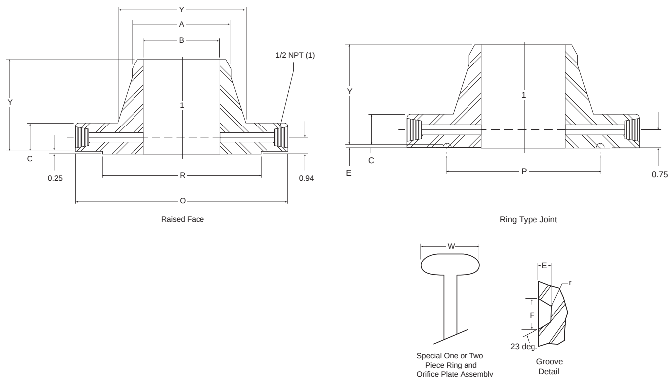
FIGURE 5. Class 600
