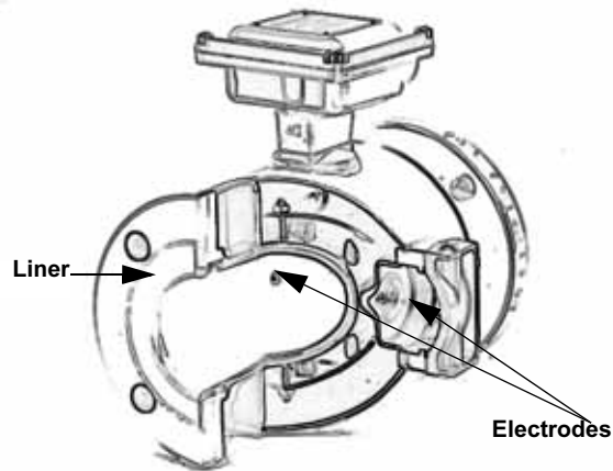
FIGURE 1. Cutaway View of a Magnetic Flowtube
