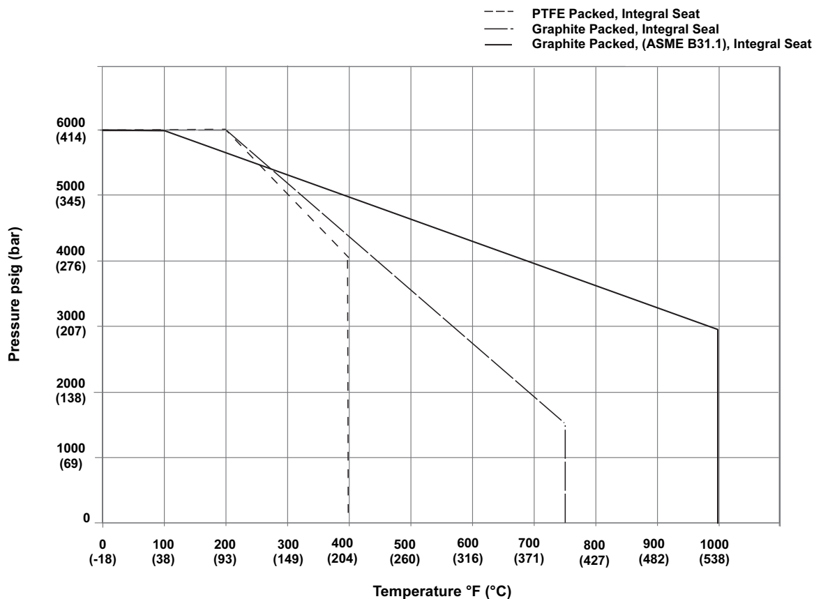
FIGURE 1. 304 Conventional Manifolds - Pressure vs. Temperature
