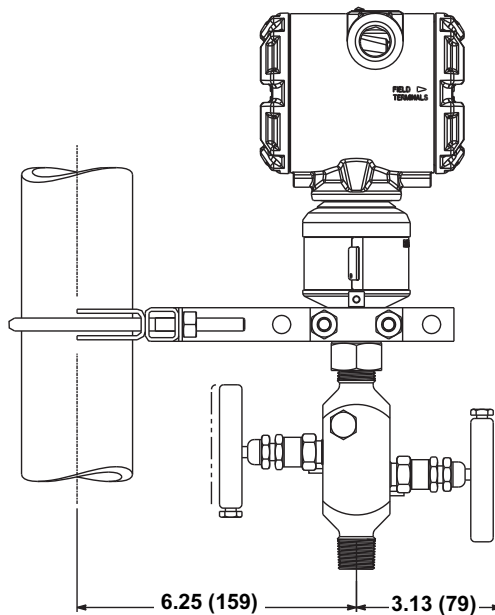
ROSEMOUNT 3051S_T
