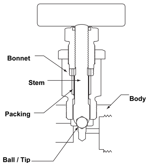
FIGURE 4. Typical Rosemount Manifold Valve
